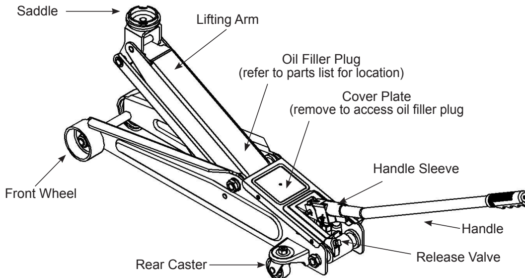
Figure 1 - High-Lift Floor Jack Nomenclature
