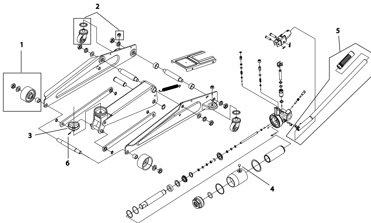
Figure 2 - Replacement Parts Illustration for Model F-2533
