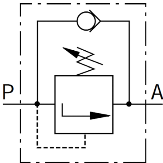
Figure 2 - CVS3 Hydraulic Symbol
