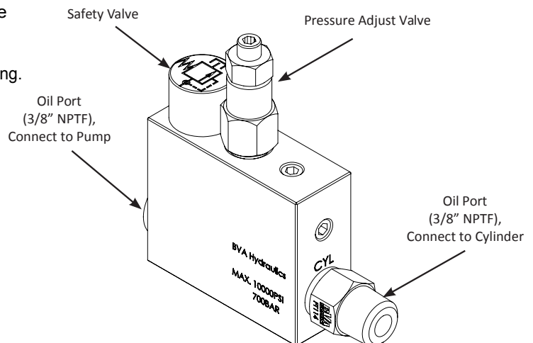
Figure 1 - CVS3 Component Nomenclature
