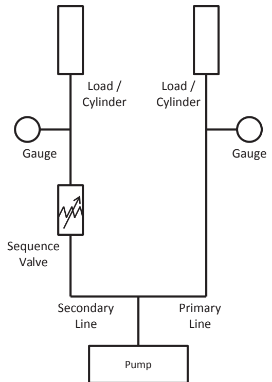
Figure 3 - Typical CVS3 Sequence Valve Connection
