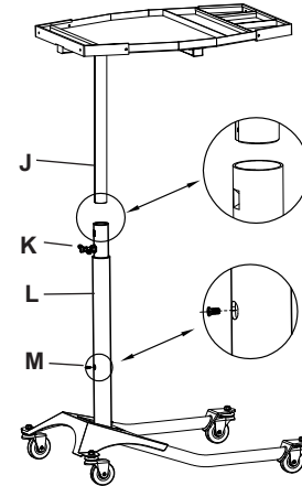
Figure 4 - Attaching Columns
