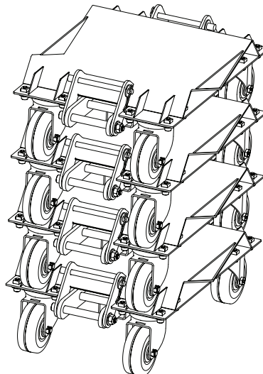
Figure 3 - Stacked Configuration
